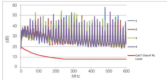
Carlisle 1E027X-8 Octax Assembly NEXT
