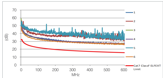
Carlisle 1E027X-8 Octax Assembly ELFEXT
