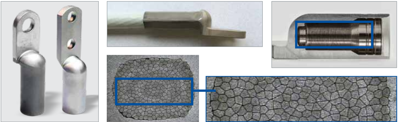
(1) One- and two-hole terminal lugs, (2) crimped terminal lug, (3) integral oxide breaker location and (4) typical cross-section example. High compaction without breaking conductor strands, offers better corrosion resistance, lower electrical resistance, and better tensile strength. » Learn more: www.carlisleit.com/products/connectors/terminal-lugs-splices
