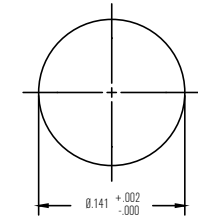
Recommended Mounting Hole
