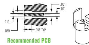
Recommended PCB Mounting Pattern
