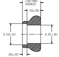
Recommended Panel Hole
